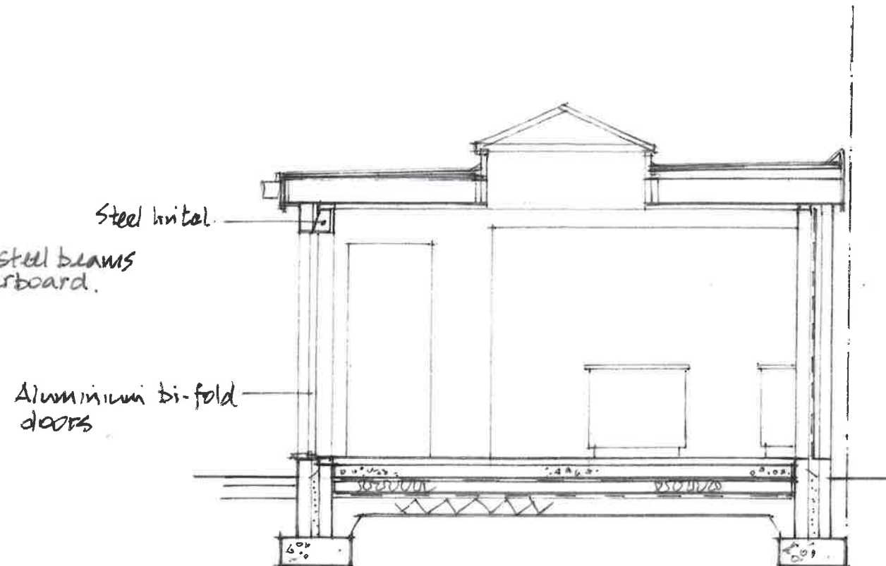
Section B-B (1:50)
