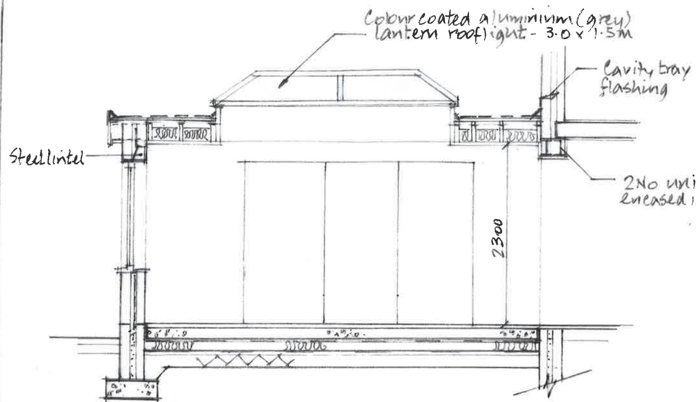
Section A-A (1:50)
