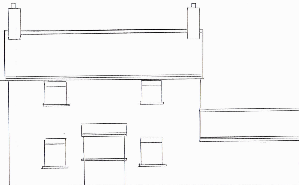
FRONT ELEVATION PROPOSED (NO CHANGES)
