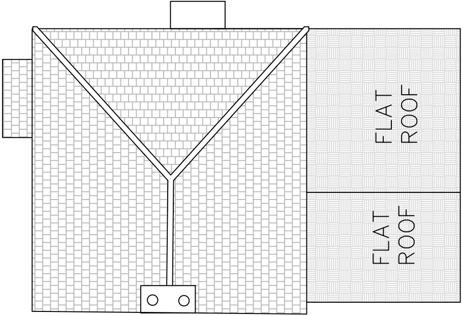
PROPOSED ROOF PLAN SCALE – 1:100 @ A3
