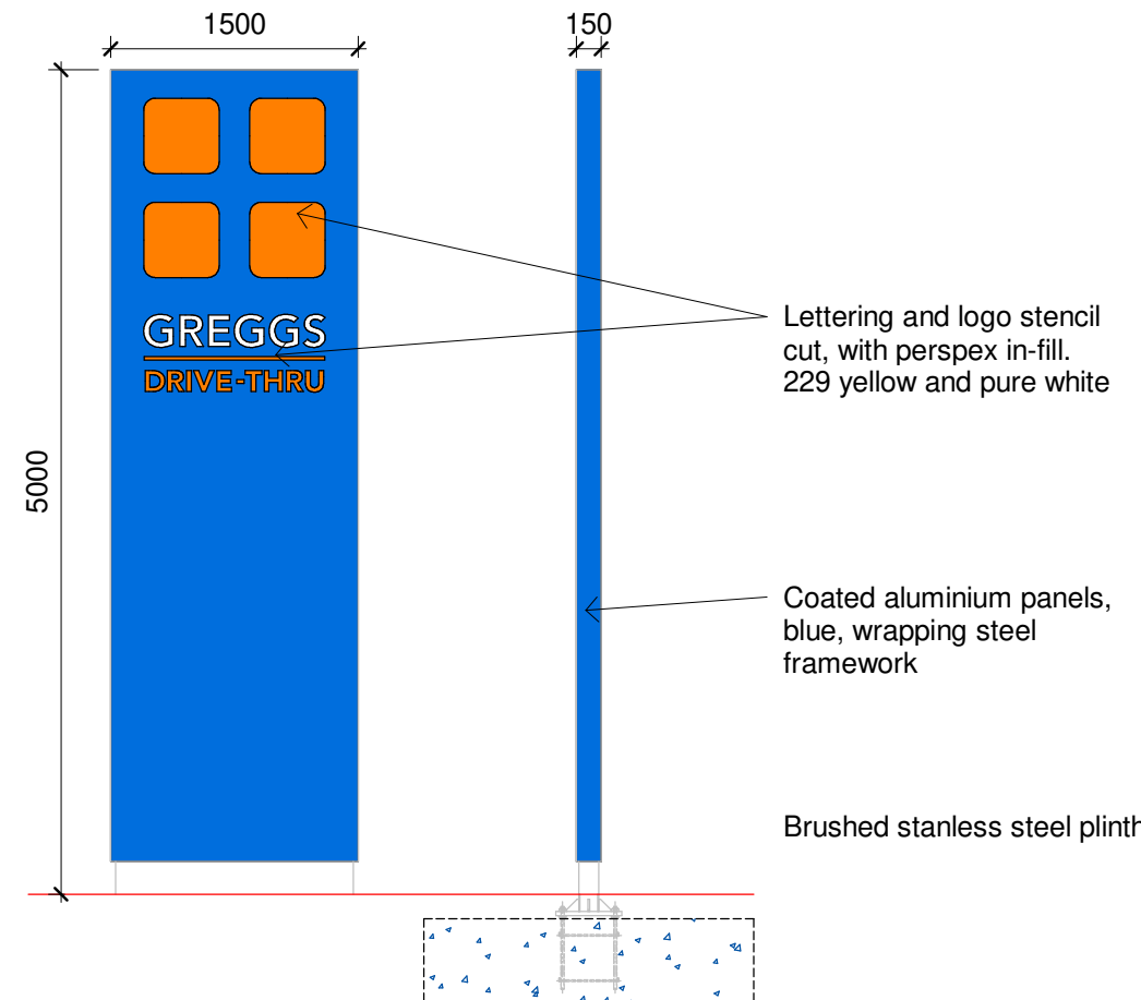
08 - 5M TOTEM SIGN
