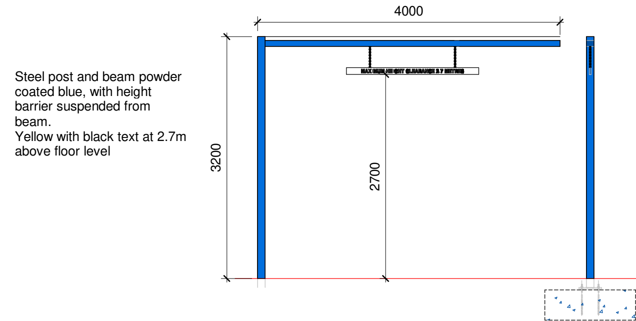
02 - HEIGHT RESTRICTION BARRIER
