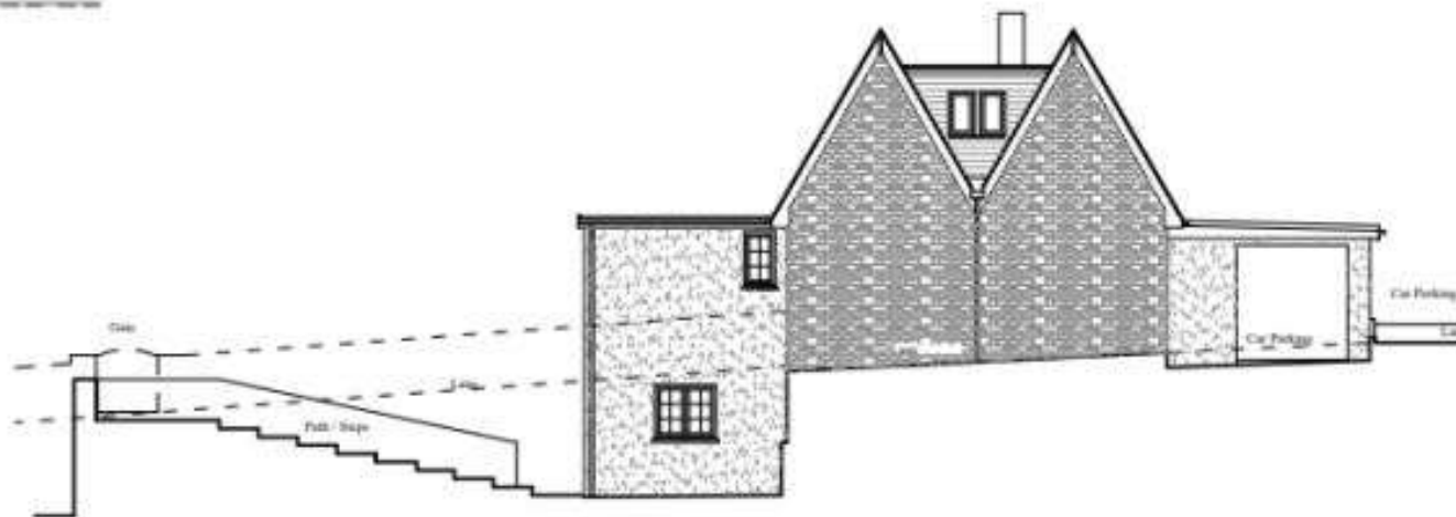
Rear Elevation
