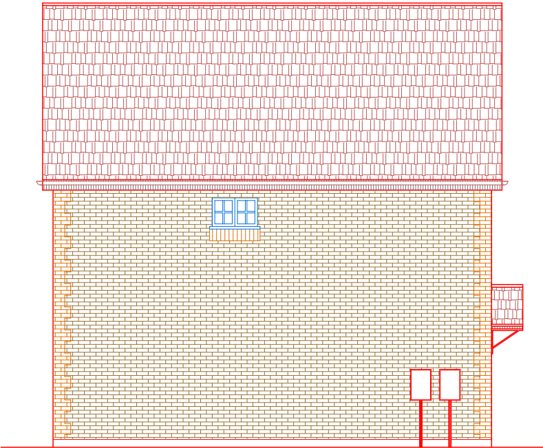
PROPOSED SIDE ELEVATION-2
