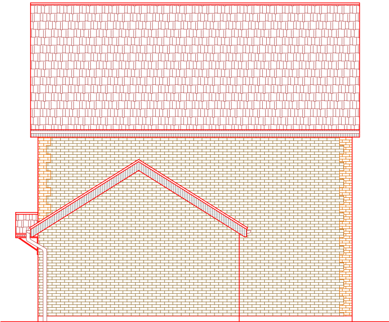
EXISTING SIDE ELEVATION-1
