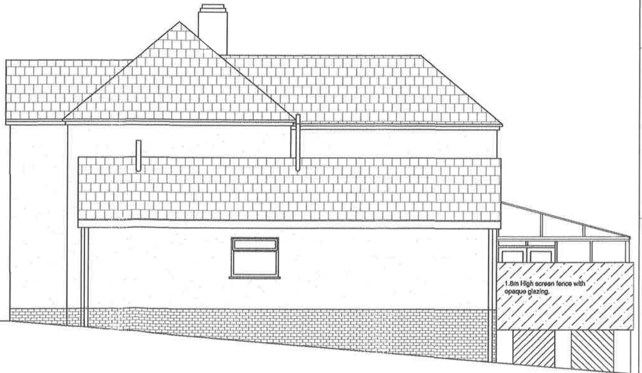
WEST ELEVATION
