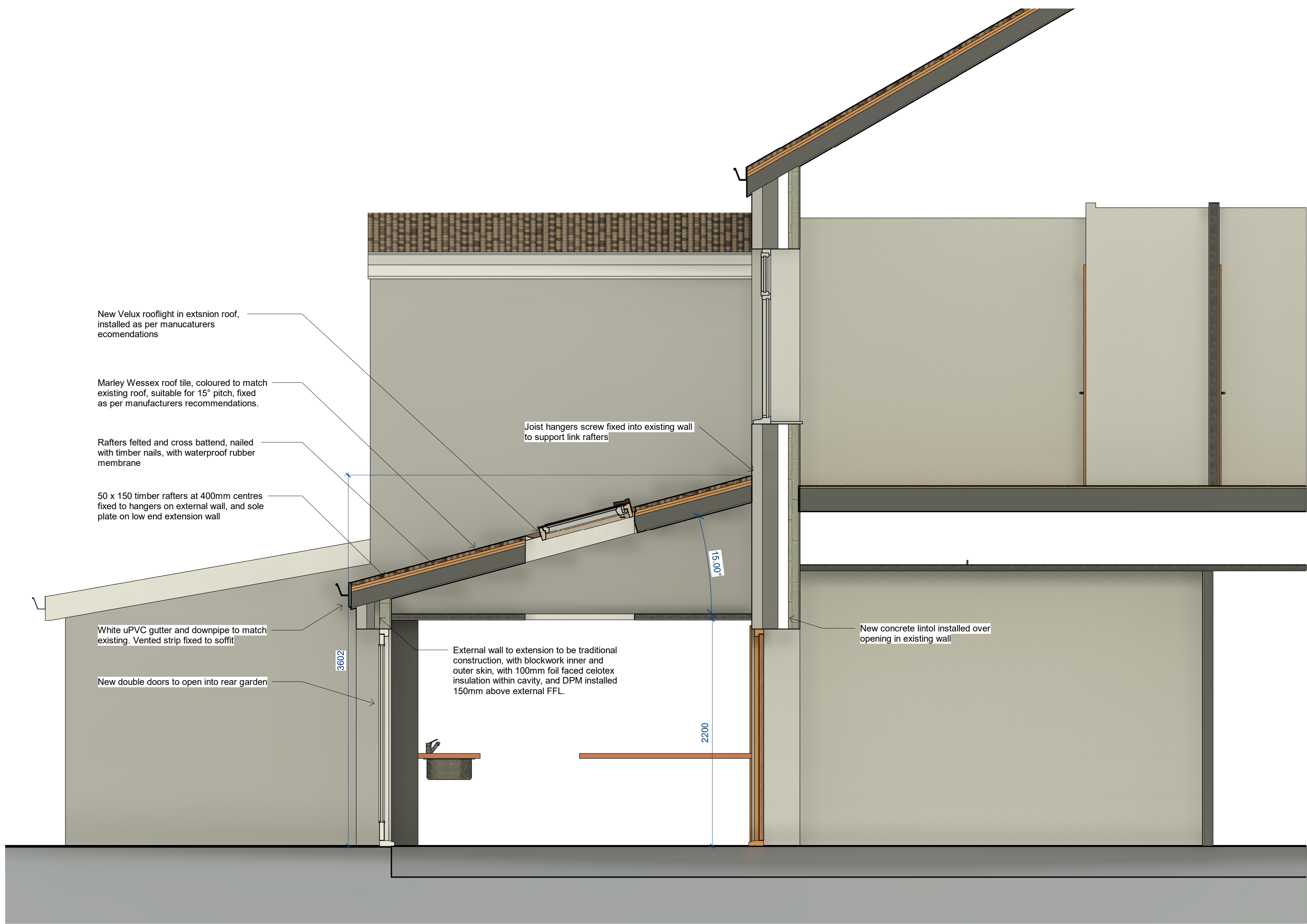
1 Proposed section through extension 1 : 25
