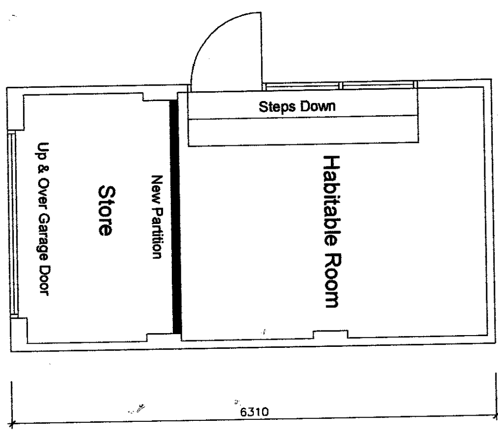
GROUND FLOOR PLAN AS PROPOSED 1:50
