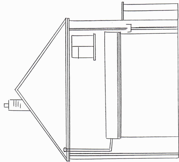
SIDE ELEVATION EXISTING
