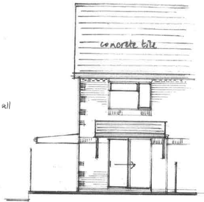
Existing Front Elevation, Rear Elevation and Side Elevation (1:100)
