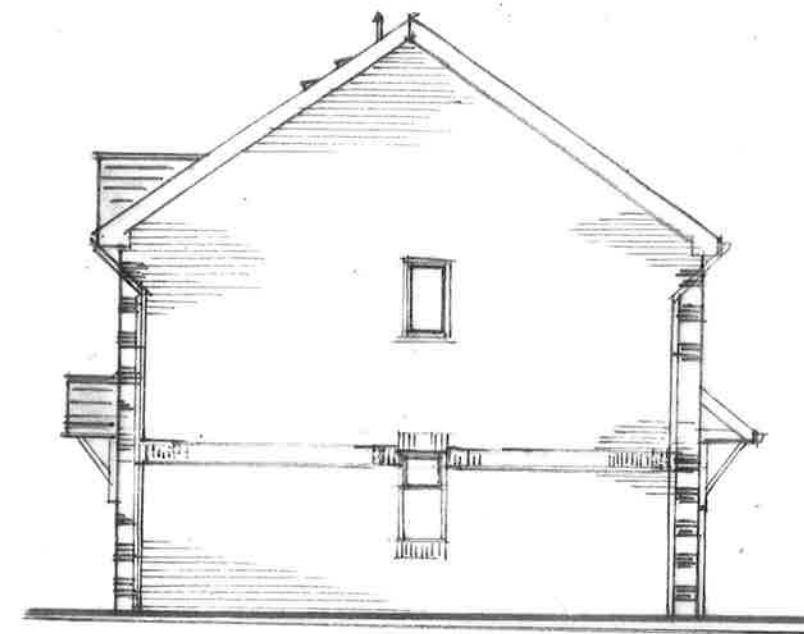
Existing Front Elevation, Rear Elevation and Side Elevation (1:100)
