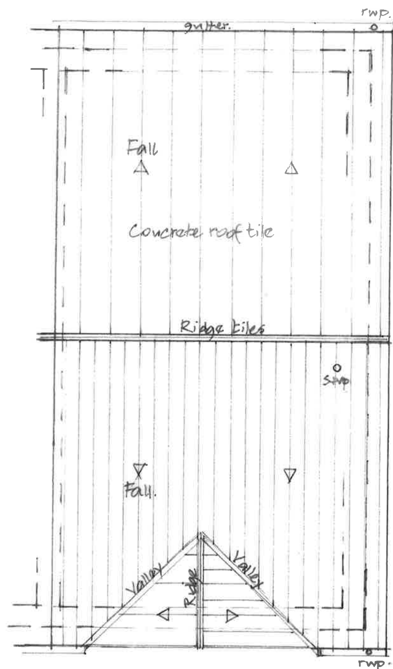
Existing Roof Plan (1:50)
