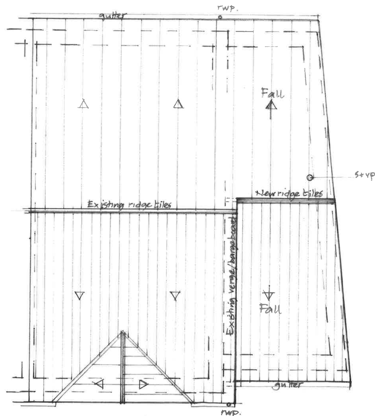
Proposed Roof Plan (1:50)
