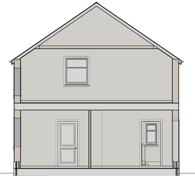
SECOND SIDE ELEVATION EXISTING
