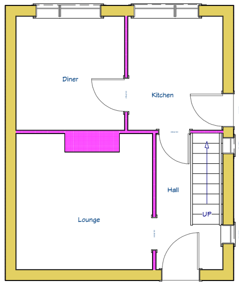
GROUND FLOOR EXISTING
