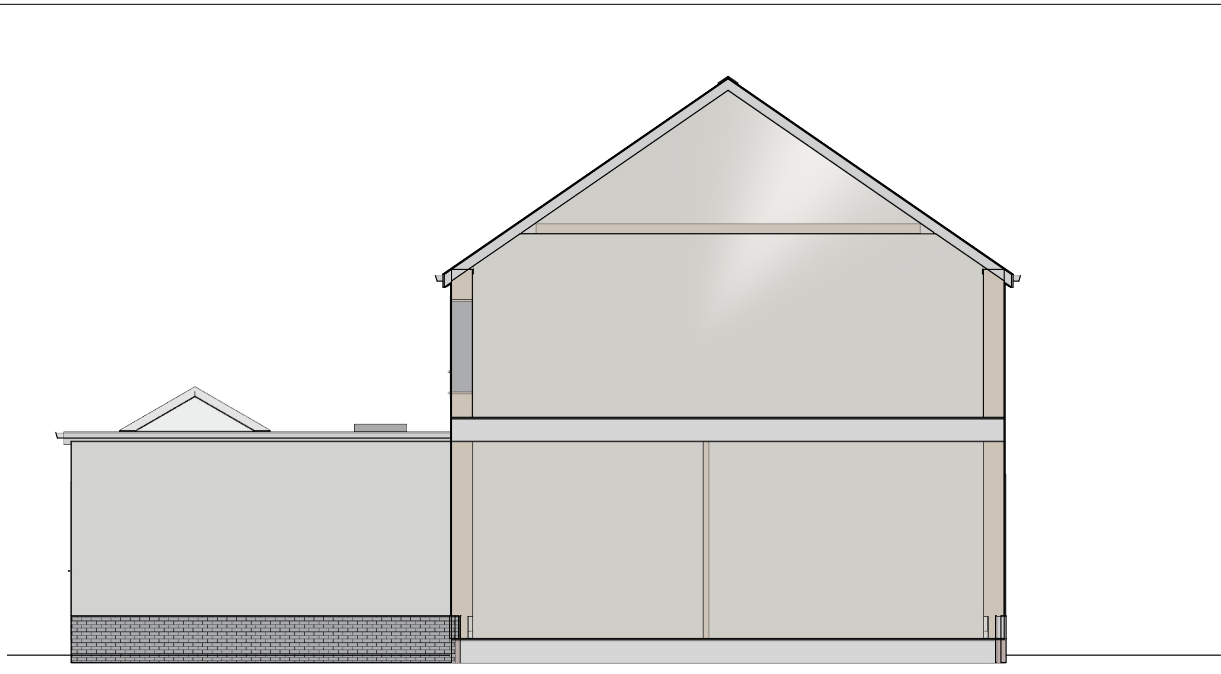
SECOND SIDE ELEVATION PROPOSED
