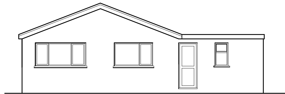
Existing Rear Elevation
