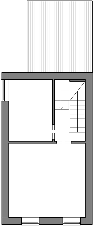
Existing First Floor Plan 1:100
