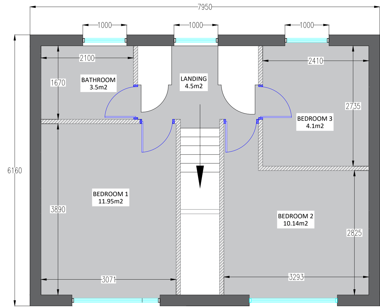
Existing First Floor Plan 1:50 @ A1
