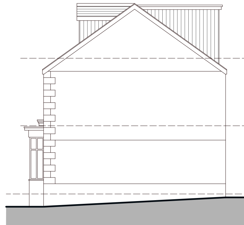
SIDE ELEVATION
