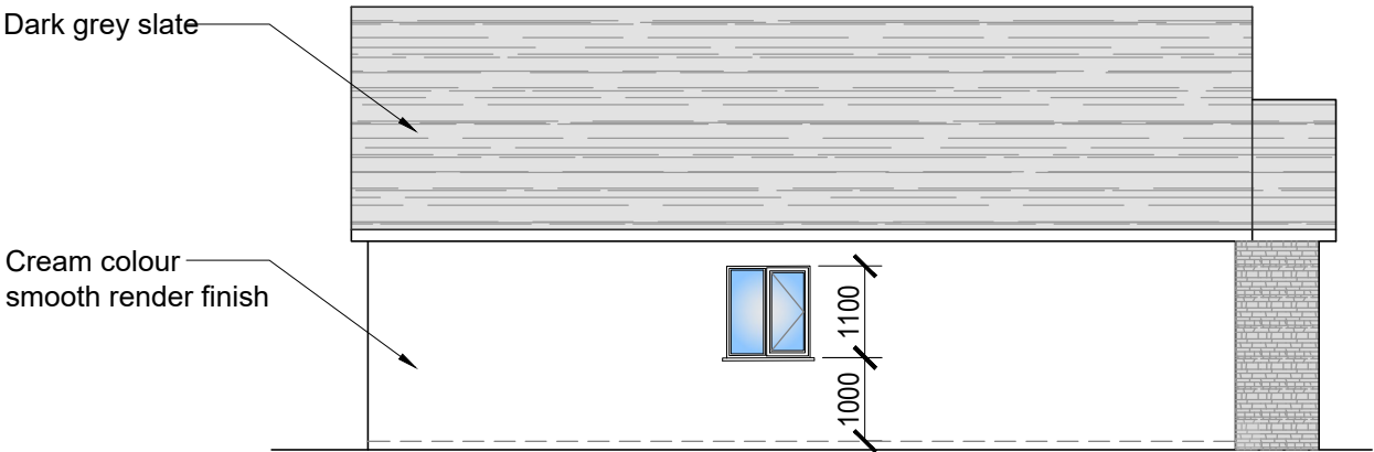
Proposed elevation on 'A' Scale - 1:100
