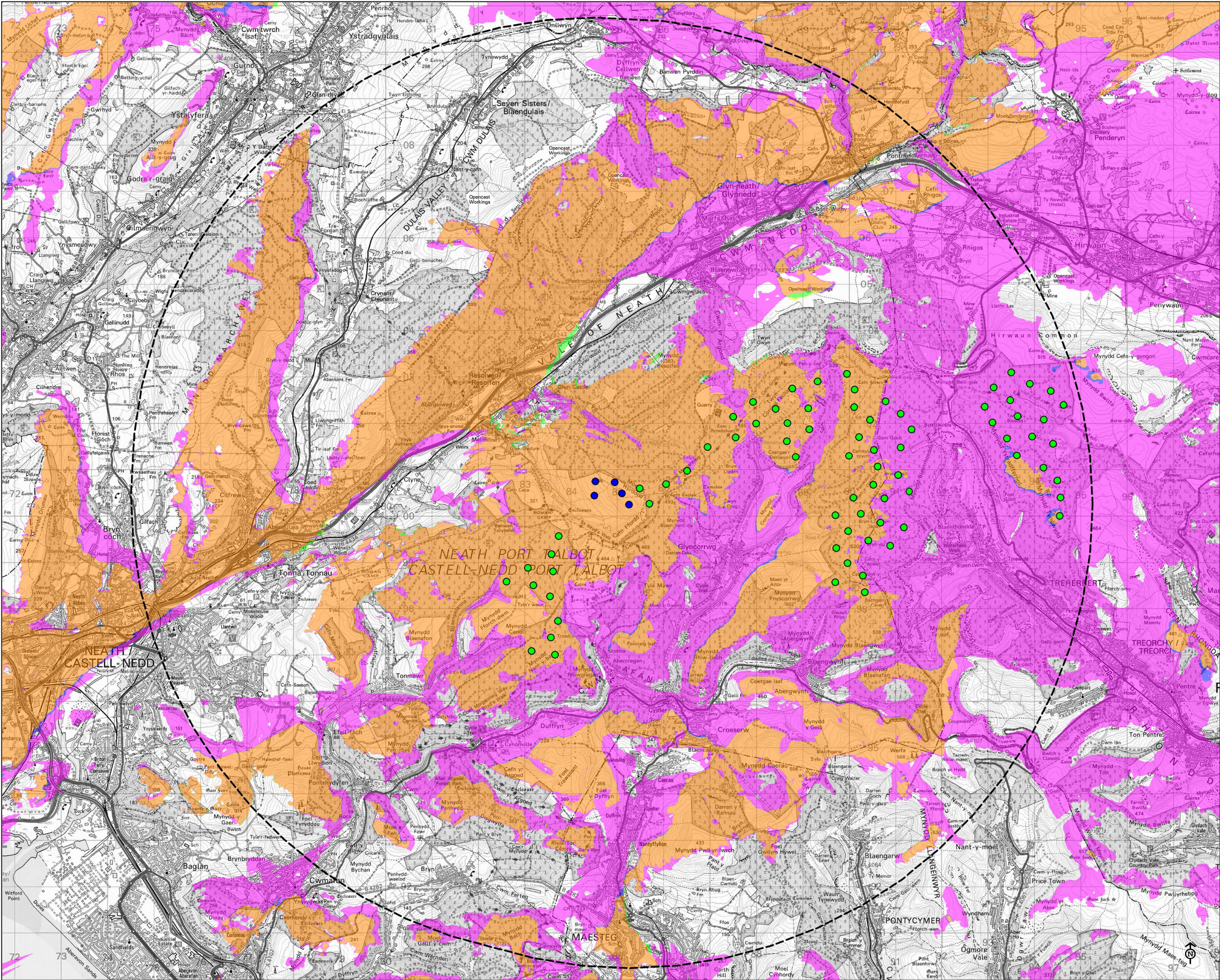
Figure A3.24A – Pen y Cymoedd Cumulative & Comparative ZTV
