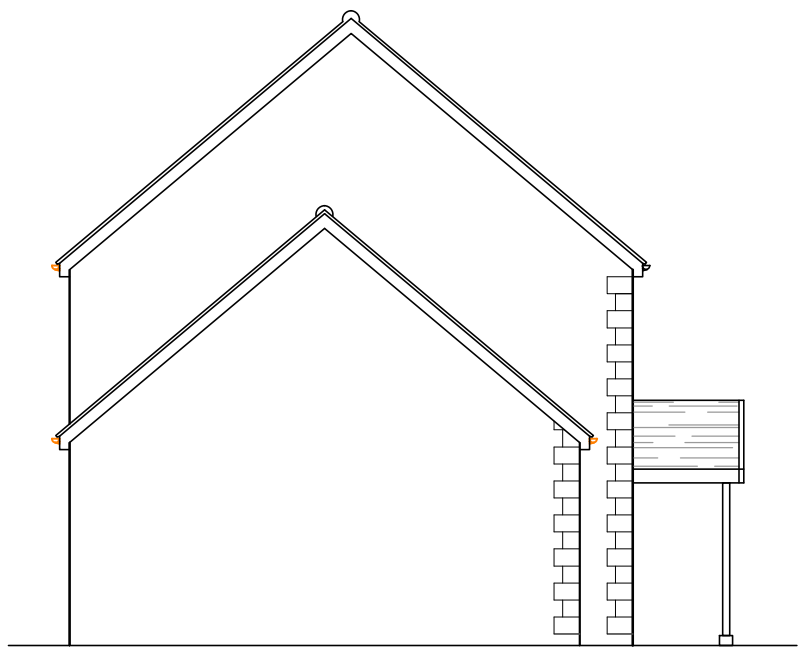
Proposed elevation on 'A' Scale - 1:100
