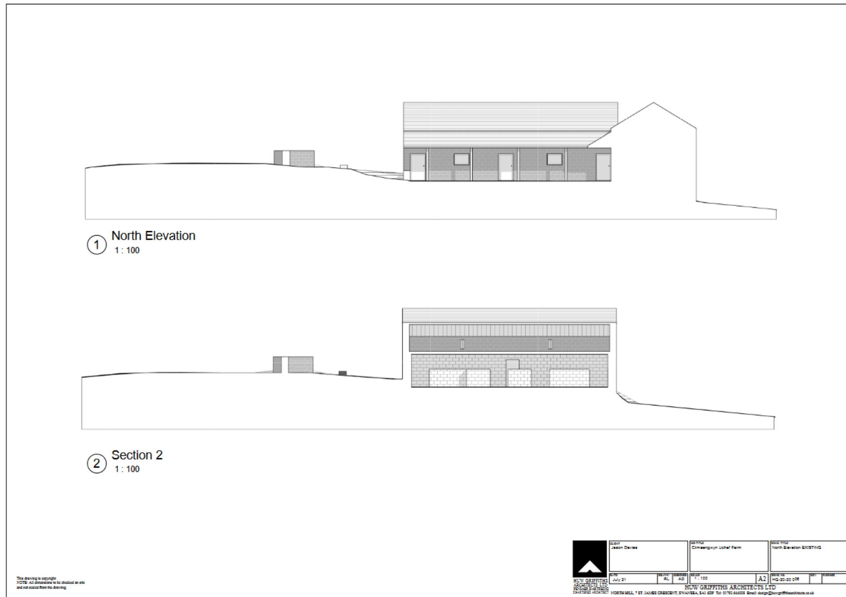
Fig. 4 – Elevation and Section as Existing
