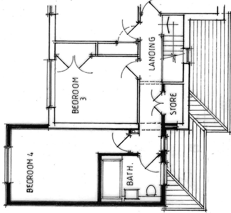
PART FIRST FLOOR PLAN
