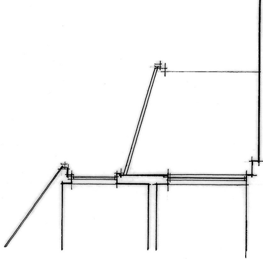
SECTIONAL SIDE ELEVATION
