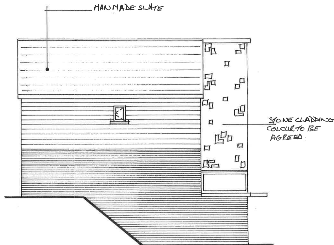
SIDE ELEVATION
