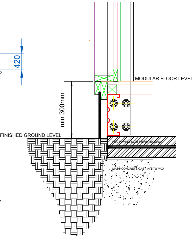
TYPICAL SECTION THRU PERIMETER FOUNDATION - 1:10
