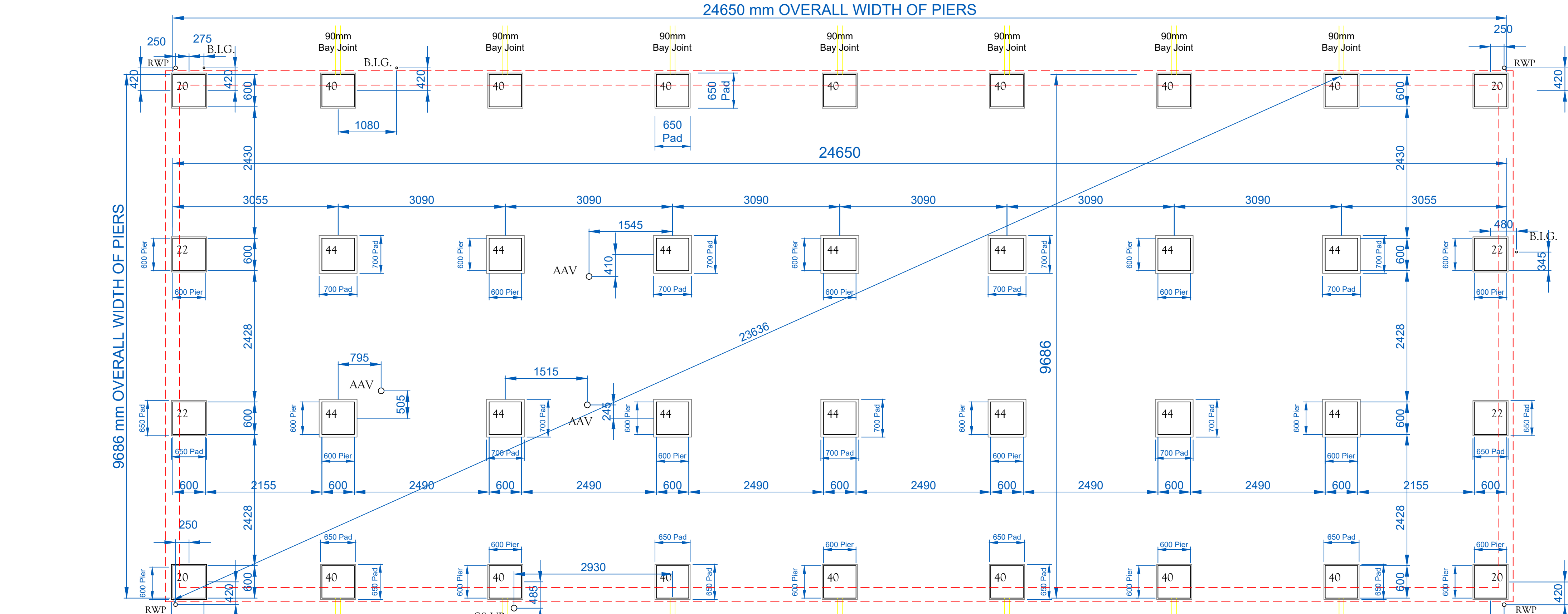
FOUNDATION PAD SETTING OUT - 1:50
