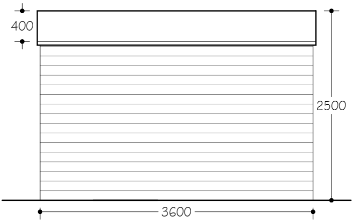
North East Elevation - 1:50
