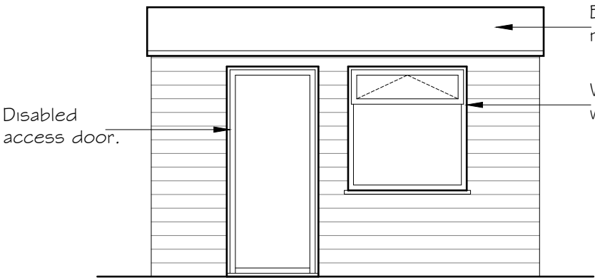
South West Elevation - 1:50
