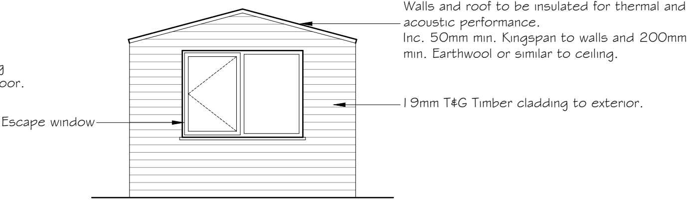
South East Elevation - 1:50
