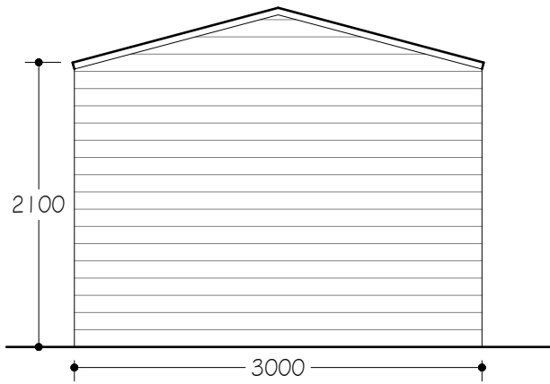
North West Elevation - 1:50
