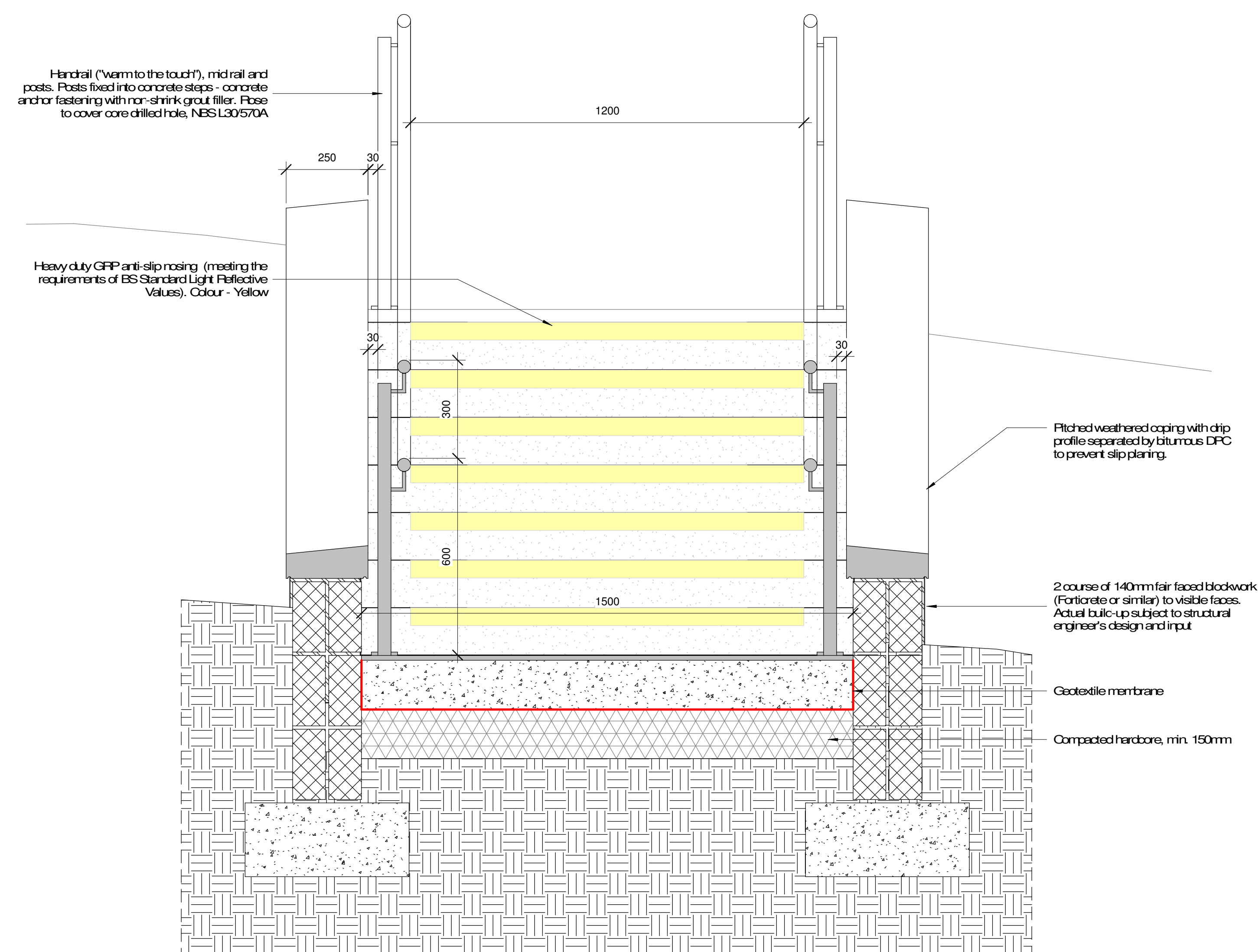
5 External Stair Cross Section-Elevation 1:10
