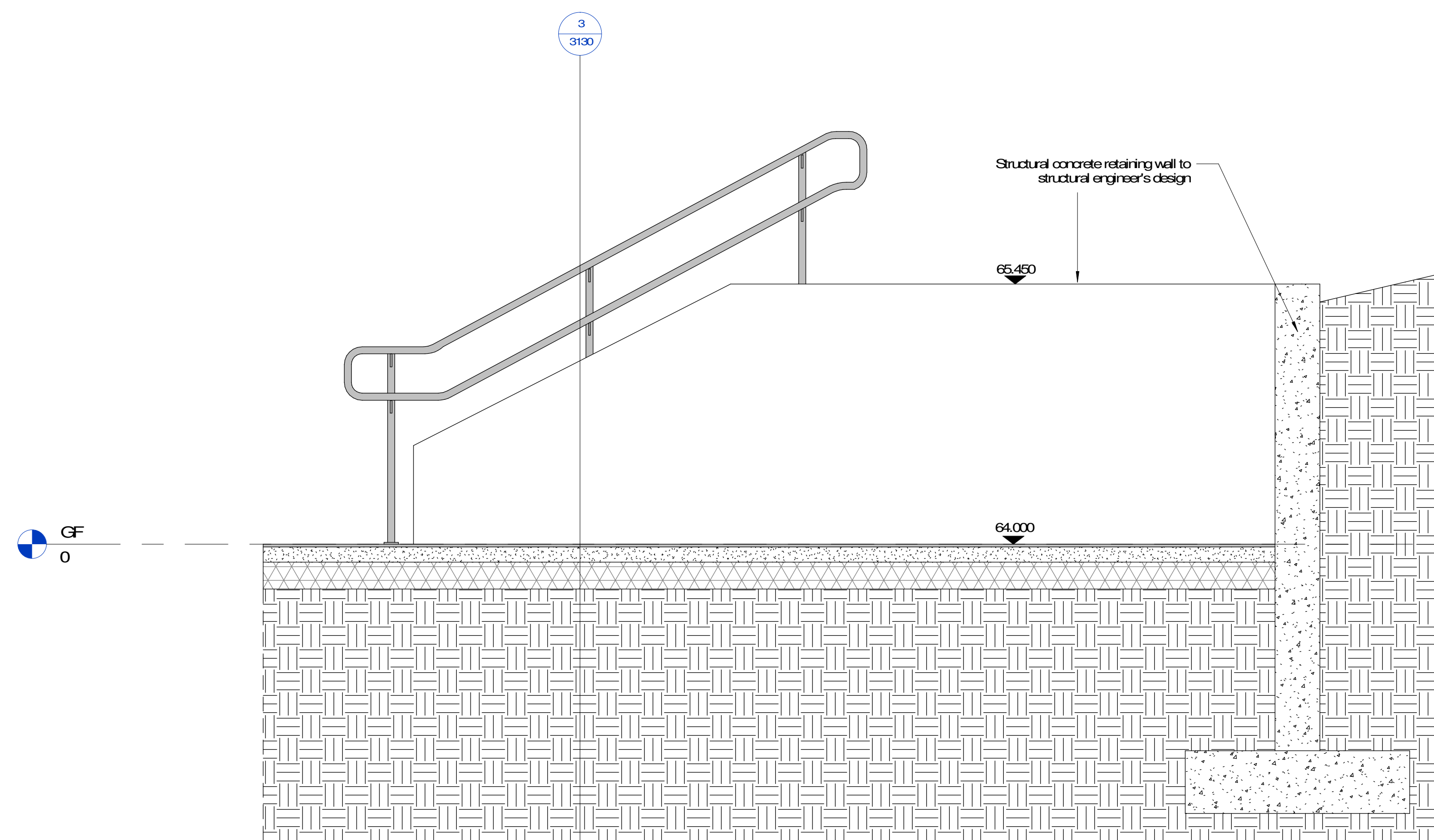
1 Retaining Wall to Stair - Elevation 1:20
