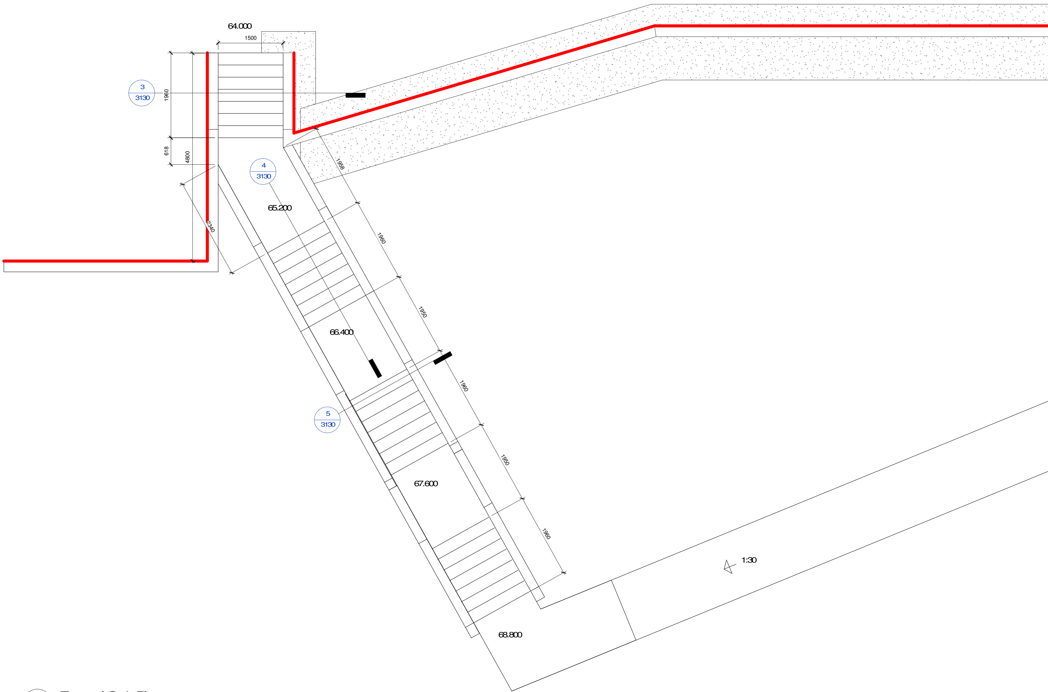
6 External Stair Plan 1:50
