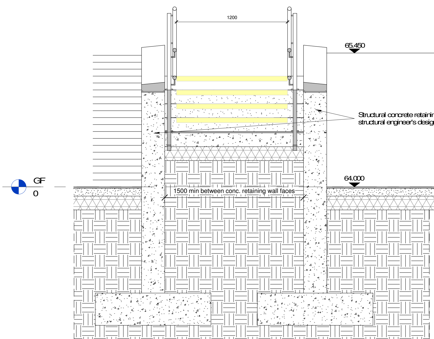
3 Retaining Walls to Stair - Section 1:20
