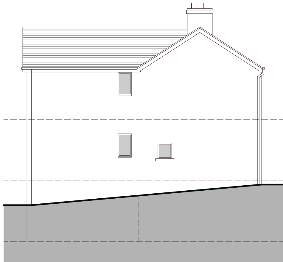
SIDE ELEVATION
