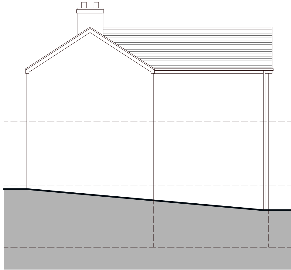
SIDE ELEVATION
