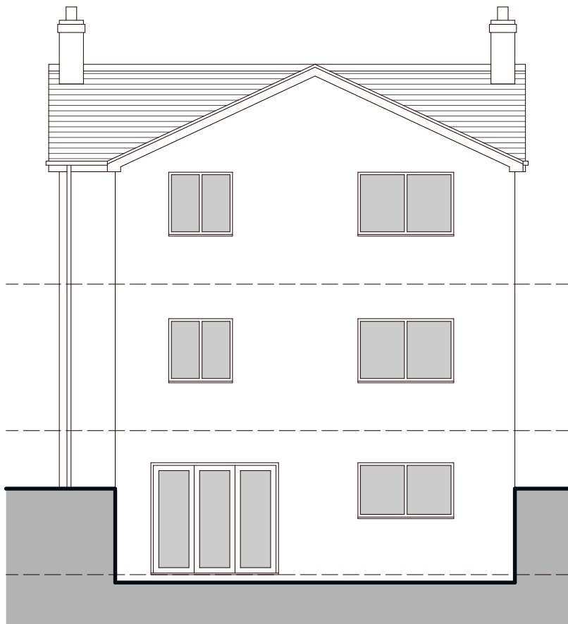
REAR ELEVATION
