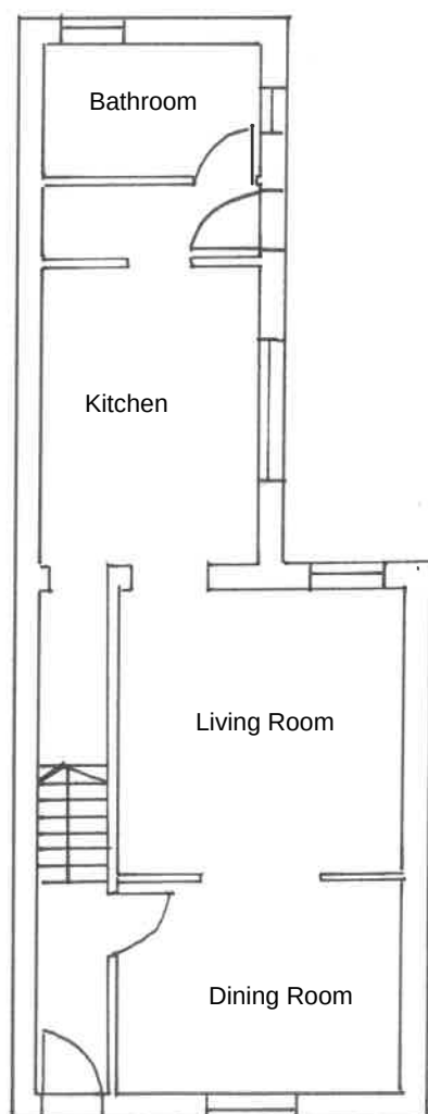
EXISTING GROUND FLOOR
