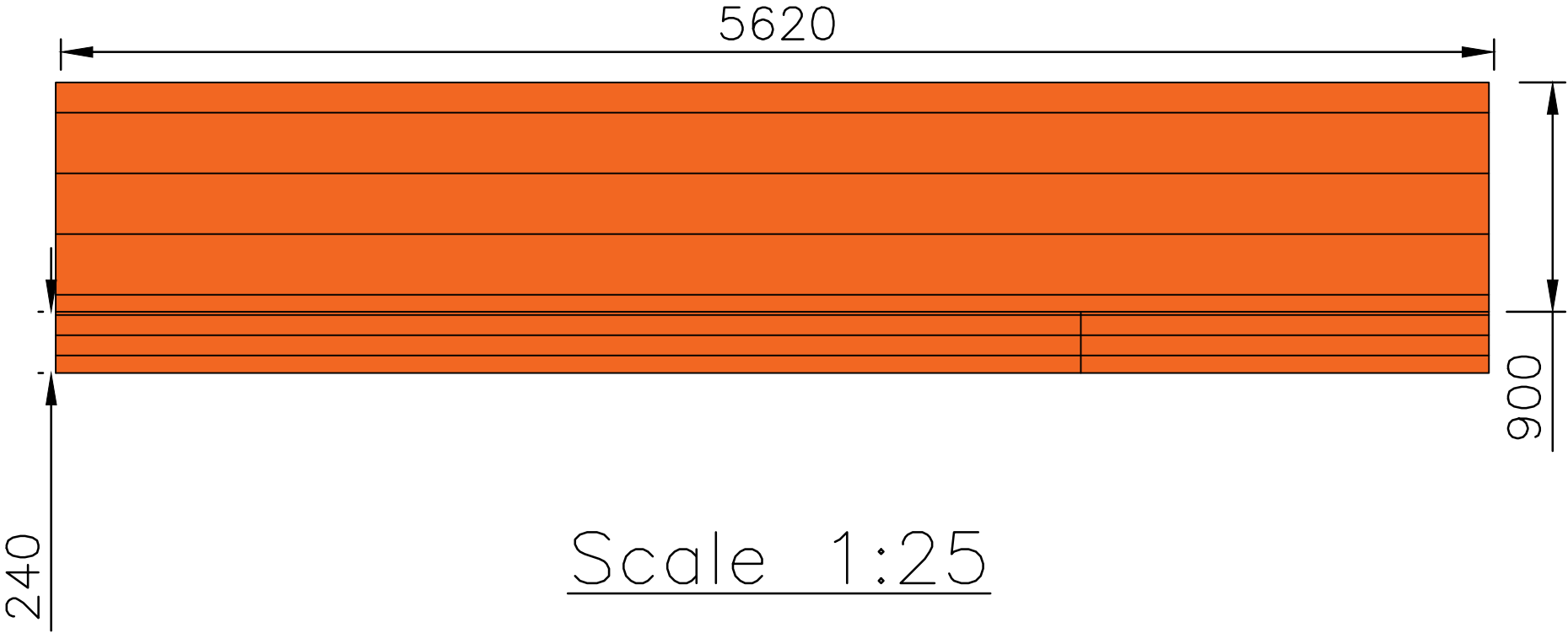
Front Side Elevation
