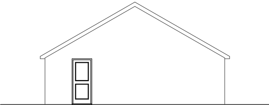
Side (South West) Elevation
