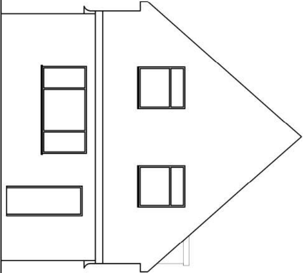
Rear Elevation
