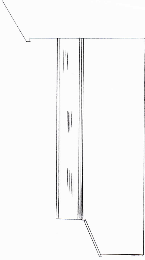
Right side elevation existing
