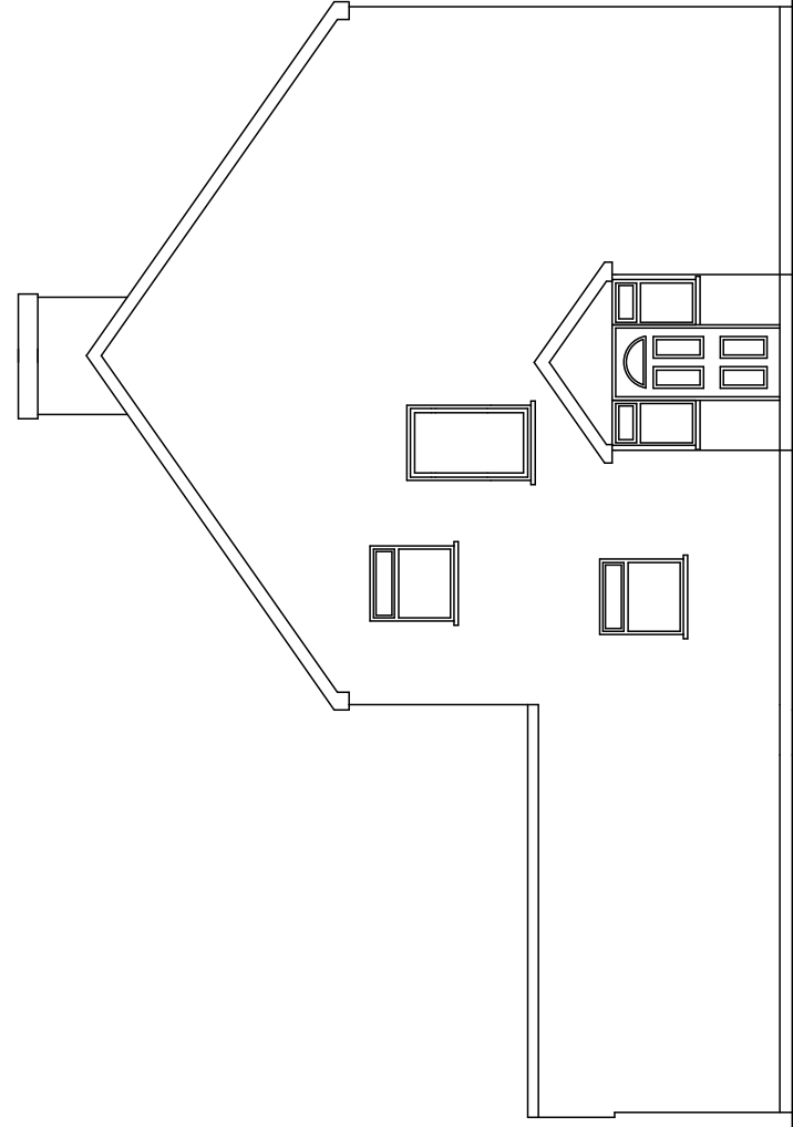
EXISTING SIDE and FRONT ELEVATIONS
