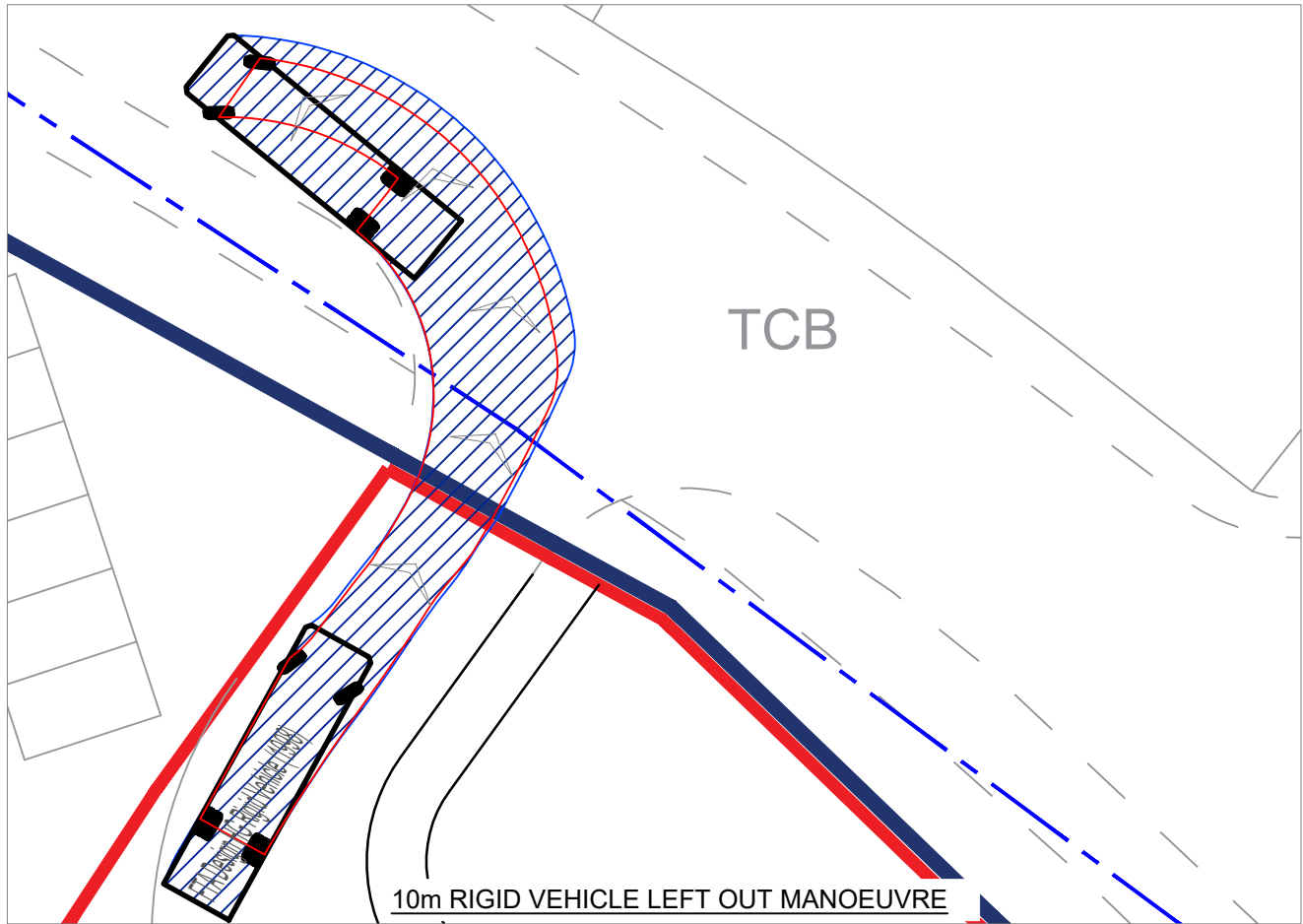
10m RIGID VEHICLE LEFT IN MANOEUVRE
