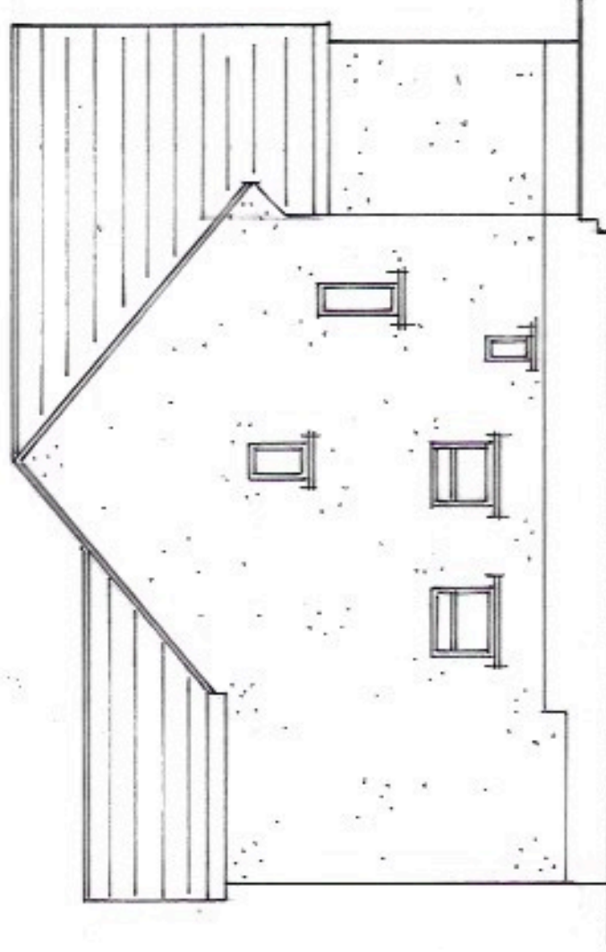
PROPOSED SIDE
