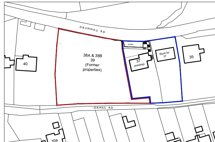
LOCATION PLAN 1:1250
