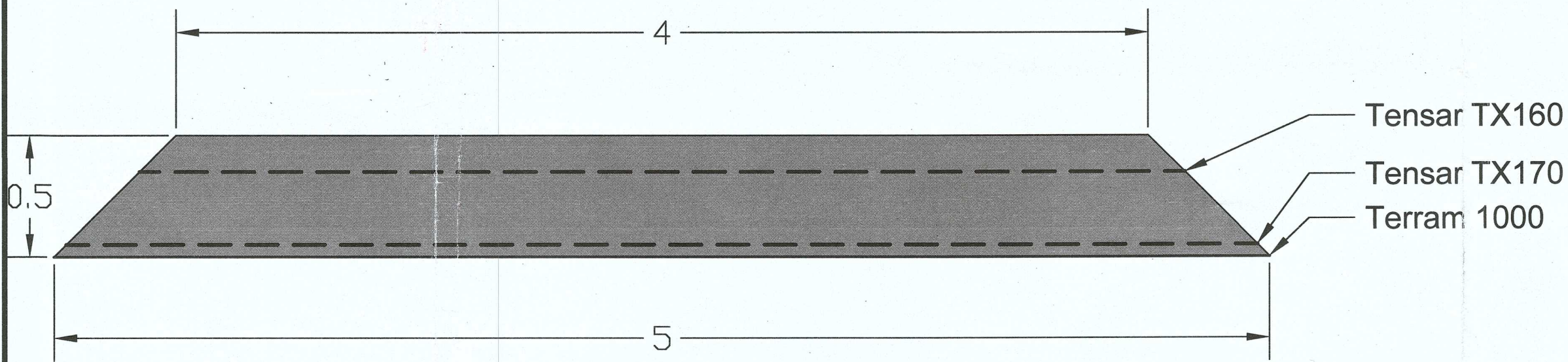
Typical Road Cross-section - road width varies depending on ground conditions encountered
