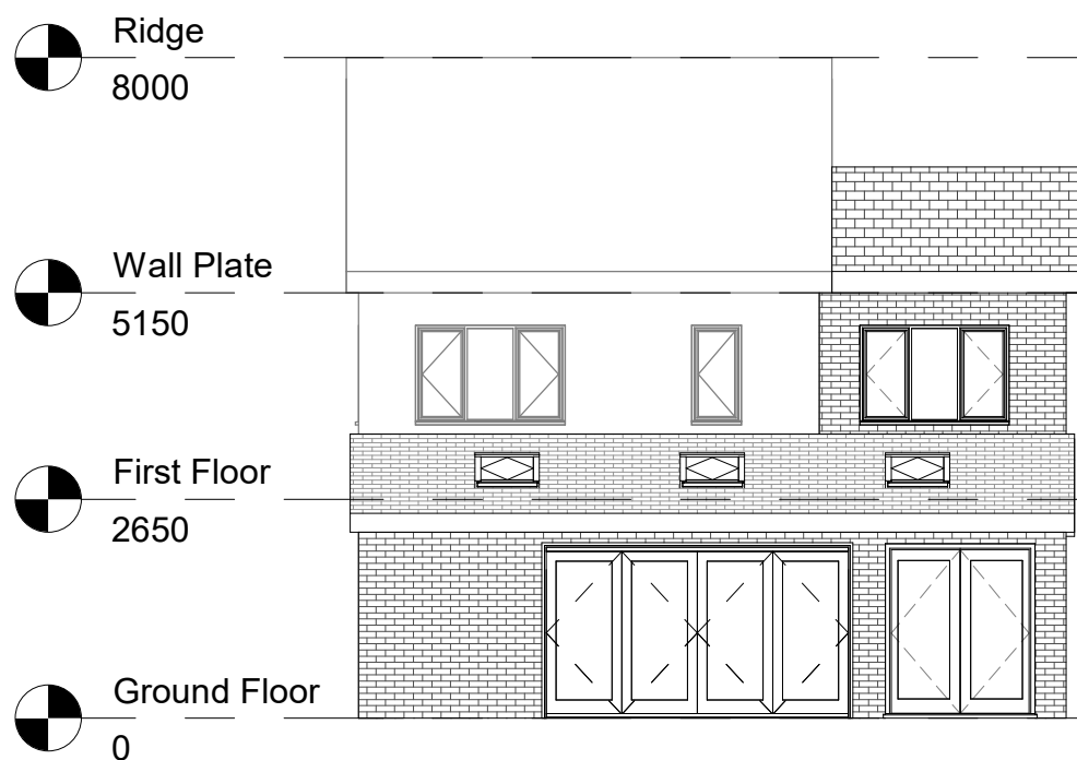
8 Proposed Rear Elevation 1 : 100
