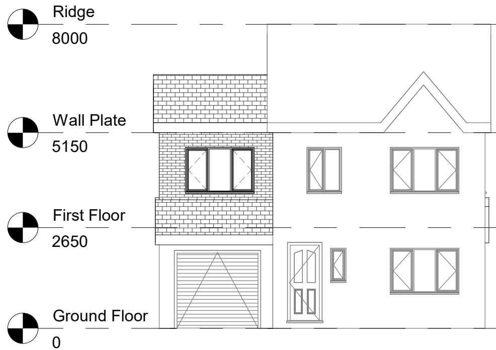
6 Proposed Front Elevation 1 : 100
