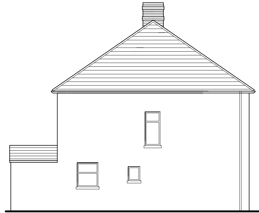
EXISTING RH SIDE ELEVATION
