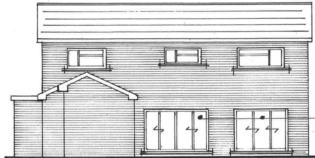
PROPOSED REAR
