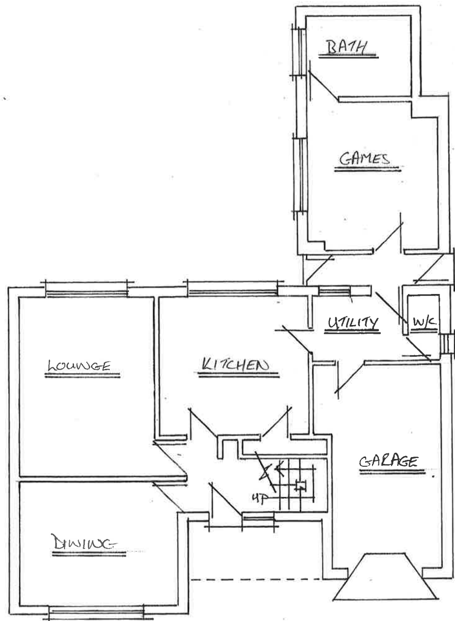
EXISTING GROUND
