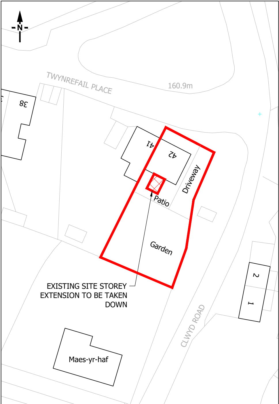
EXISTING BLOCK PLAN SCALE 1:500
