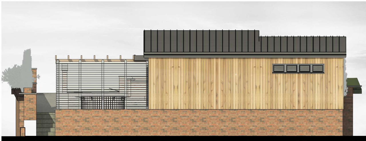
SOUTH ELEVATION (no context) 1 : 100
