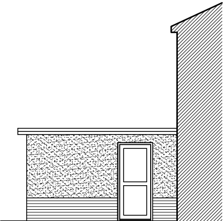
Existing Side Elevation
