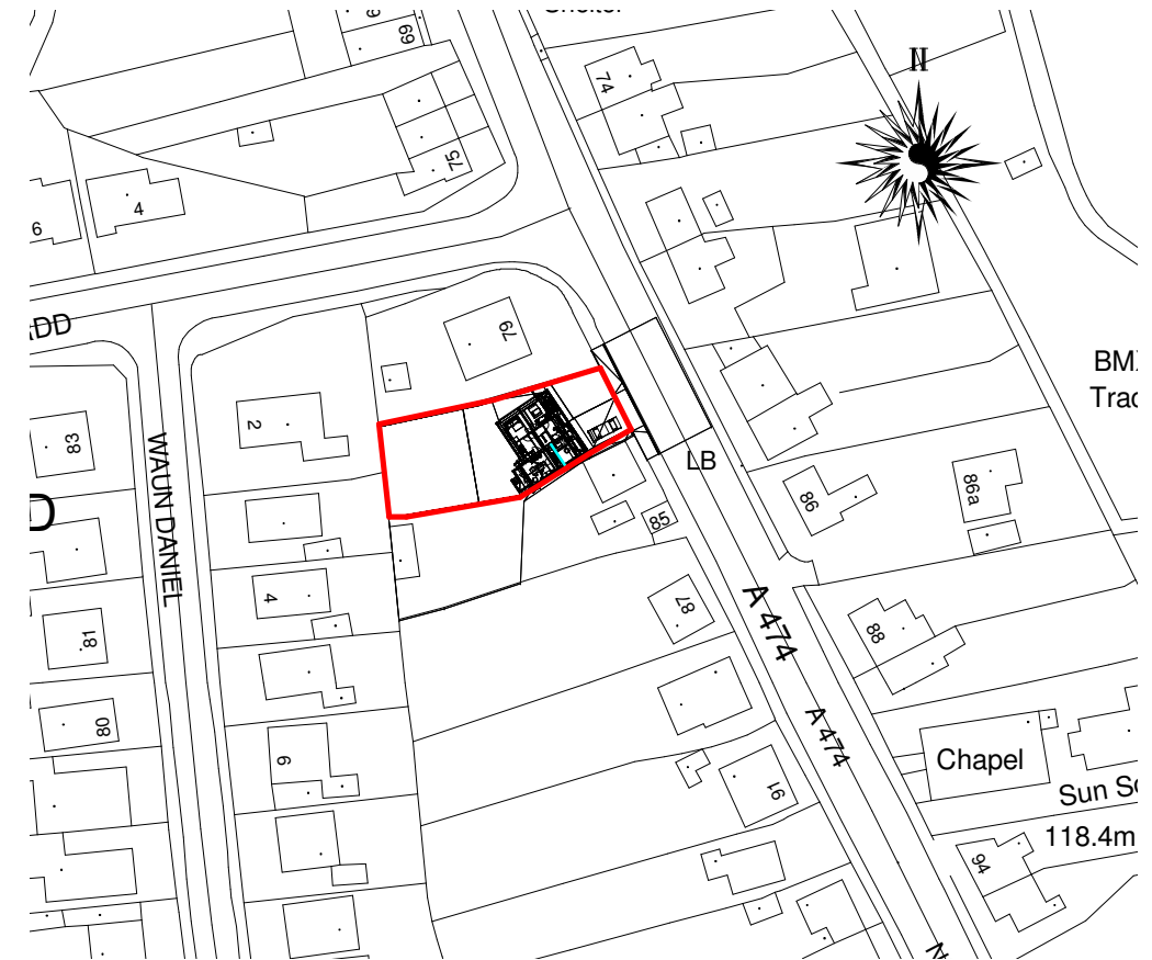
LOCATION PLAN 1 : 1250
