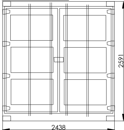
20ft Shipping Container - Door Elevation
