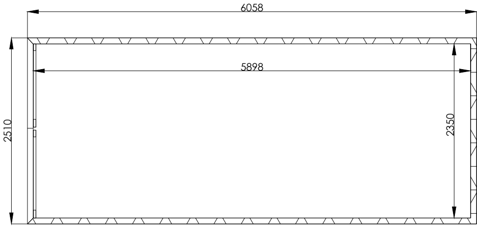
20ft Shipping Container - Plan
