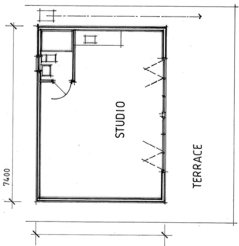
PLAN
